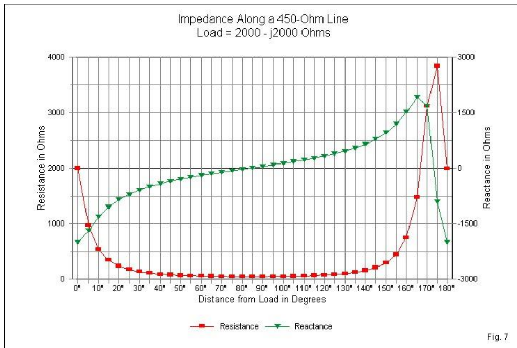
Fig. 7 shows one example of the transformation and applies to 450-Ohm transmission line and a feedpoint impedance of 2000 - j2000 Ohms. This impedance is similar to some values in Table 2 .
