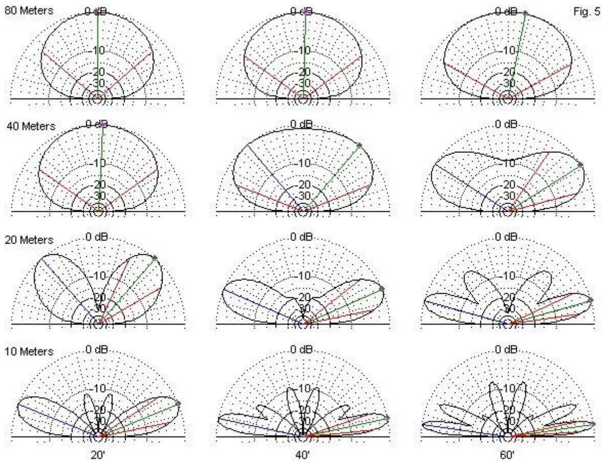
Selected Elevation Patterns: 135' Doublet on 80, 40, 20, and 10 Meters (Pattern taken along the line of maximum gain.)
