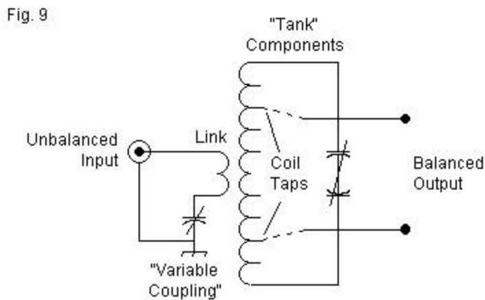
One Version of a Link-Coupled HF Antenna Tuner
